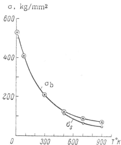
Fig. 4. Temperature dependence of the compressive strength \sigma_b and the yield point \sigma_s of beryllium single crystals on compression at right angles to the basal plane (0001).
